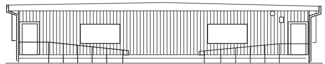
FRONT ELEVATION
